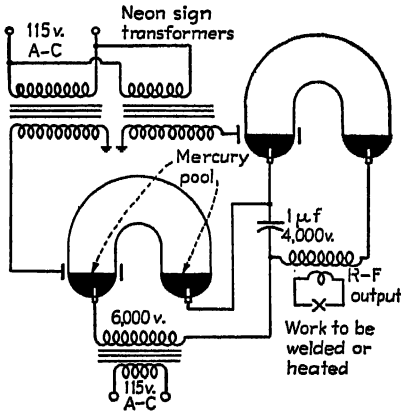
Electronic circuit used for one form of high-frequency welding.
